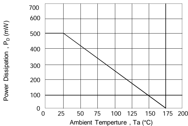
Derating Curve
