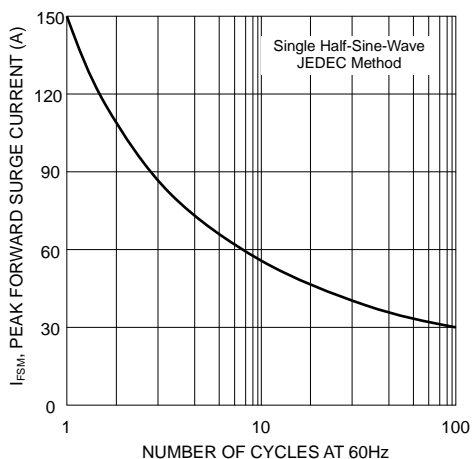
Fig. 3 Forward Surge Current Derating Curve
