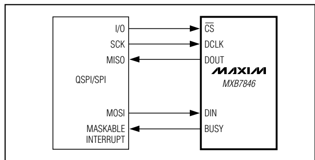
Figure 14. QSPI/SPI Interface
