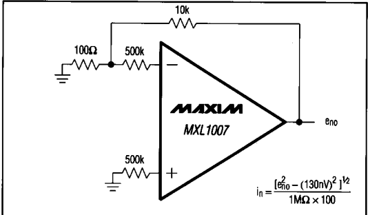
Figure 2. Current-Noise Test Circuit
