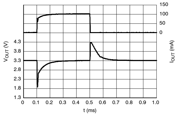
Figure 31. Load Transients, 3.3 V Version, I_{OUT} = 1 - 100 mA, t_R = t_F = 0.5 \mu s, V_{IN} = 4.3 V
