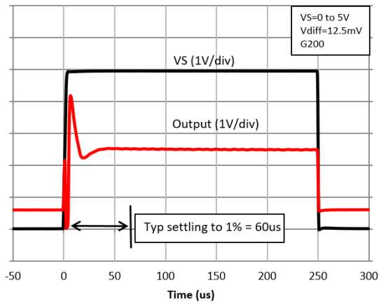
Figure 23. Start-Up Response
