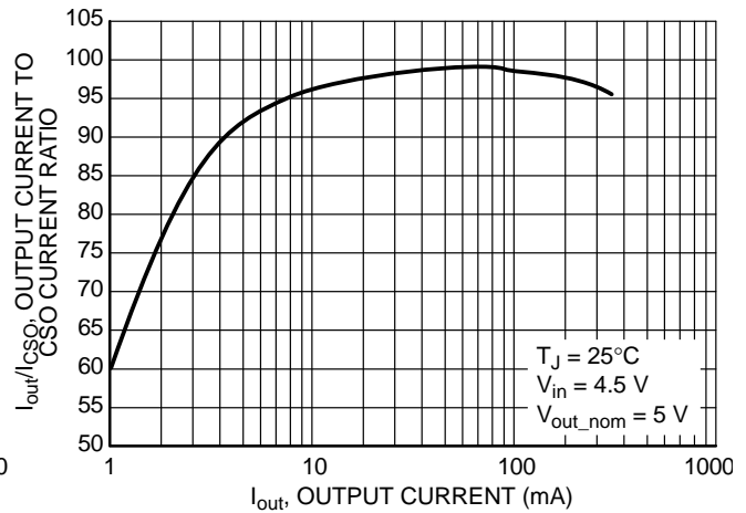
Figure 12. Output Current to CSO Current Ratio vs. Output Current in Dropout
