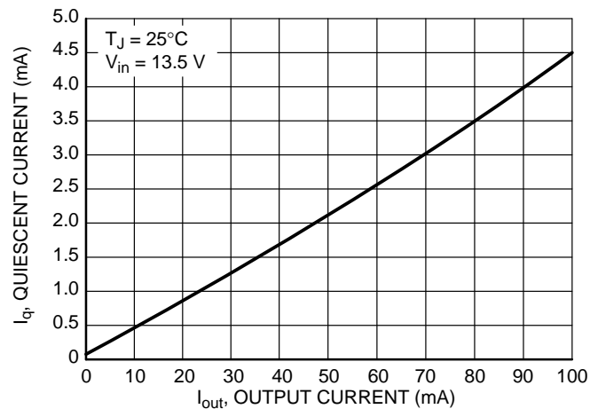
Figure 14. Quiescent Current vs. Output Current (Low Load)
