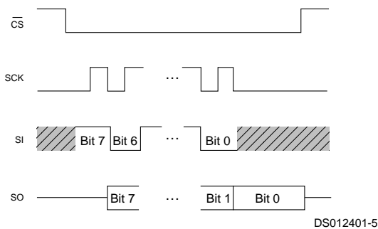
FIGURE 4. SPI Protocol
