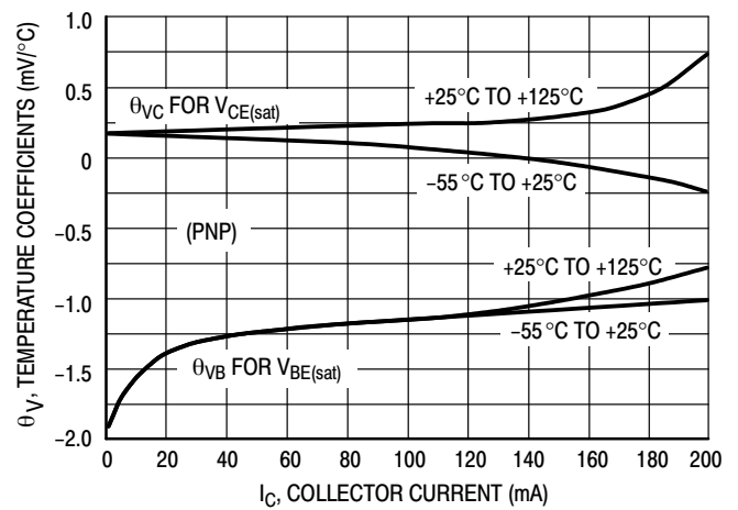
Figure 32. Temperature Coefficients
