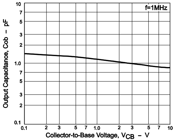
Figure 5. C_{ob} - V_{CB}
