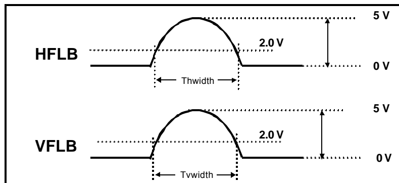
Figure 2. HV Fly-Back Signal
