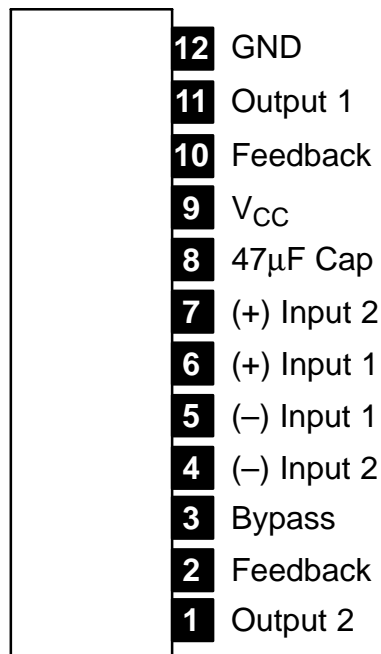
Pin Connection Diagram (Front View)
