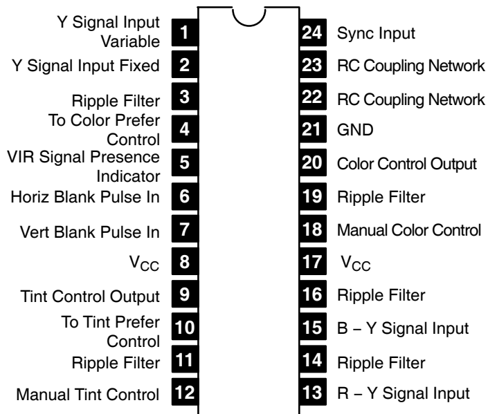
Pin Connection Diagram (Front View)
