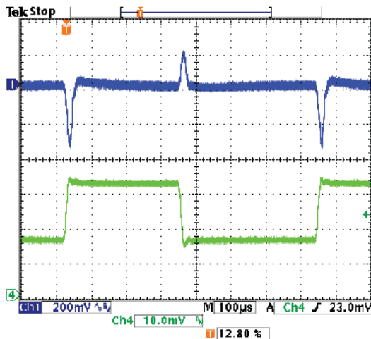
OKX2-T/16-D12 Step Load Transient Response (Vin=12V, Vout=5V, Cin=1000μF, Cload=0, Iout=8A to 16A to 8A) Trace1=Vout, 200 mV/div., Trace4=Iout, 5A/div.
