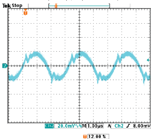
OKX2-T/16-D12 Output Ripple and Noise (Vin=12V, Vout=5V, Iout=16A, Cin=1000μF, Cload=1μF // 10μF, ScopeBW=100MHz)
