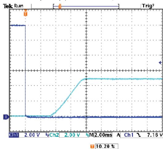
OKX2-T/16-D12-C On/Off Enable Startup Delay (Vin=12V, Vout=5V, Iout=16A, Cin=1000μF, Cload=1μF // 10μF) Trace 1=Enable In, Trace2=Vout
