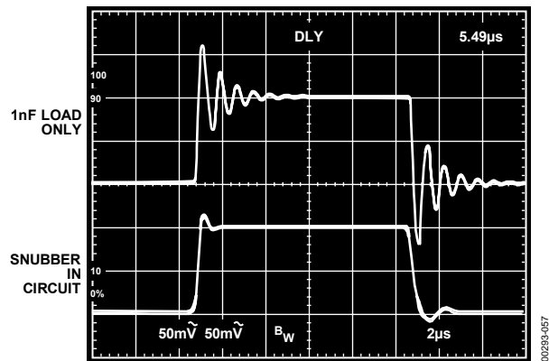
Figure 57. Overshoot and Ringing Is Reduced by Adding a Snubber Network in Parallel with the 1 nF Load
