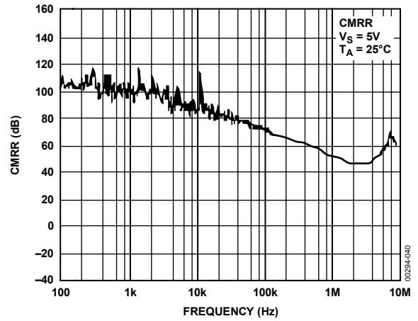
Figure 35. CMRR vs. Frequency, V_S = 5V
