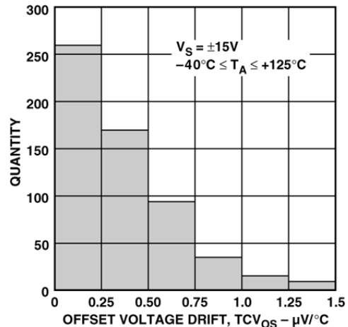
FIGURE 5. INPUT OFFSET VOLTAGE DRIFT DISTRIBUTION
