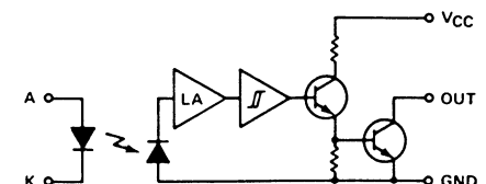
OPI128 (Open-Collector Output) Inverter
