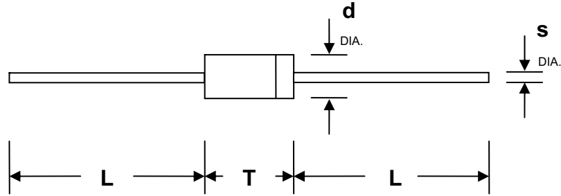
DO-201AL/DO-41
