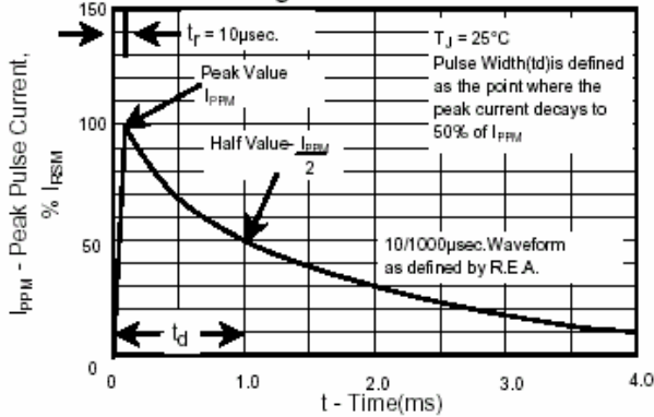
Fig.3 - Pulse Waveform
