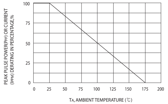
FIG.2-PULSE DERATING CURVE
