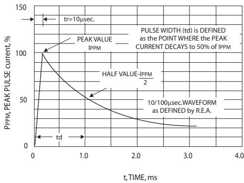
FIG.3-PULSE WAVEFORM
