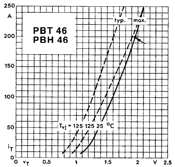
On-state characteristics
