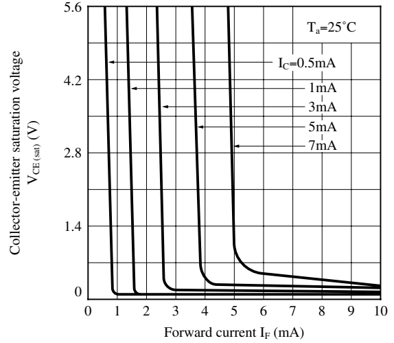
Fig.14 Collector-emitter Saturation Voltage vs. Forward Current
