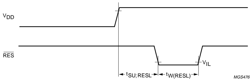
Fig.16 Reset timing.
