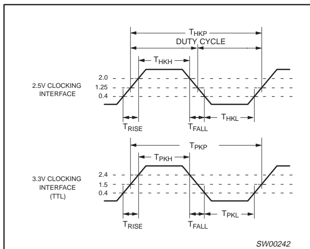
Figure 3. 2.5V/3.3V Clock waveforms
