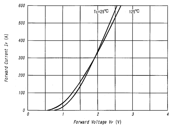
Fig. 8 Forward Characteristics of Free Wheeling Diode (Typical)
