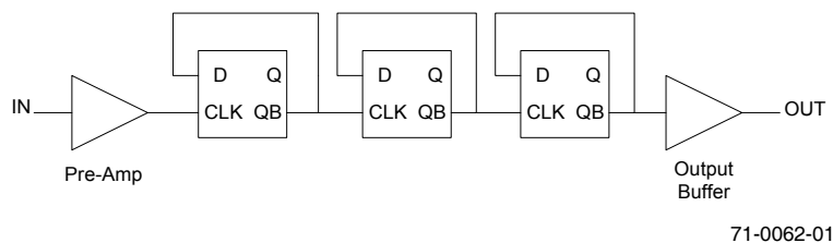
Figure 1. Functional Diagram
