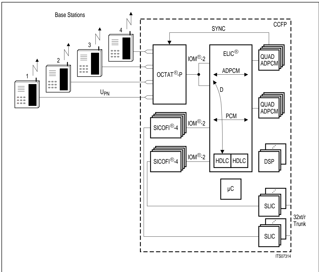
Figure 21 DECT Application
