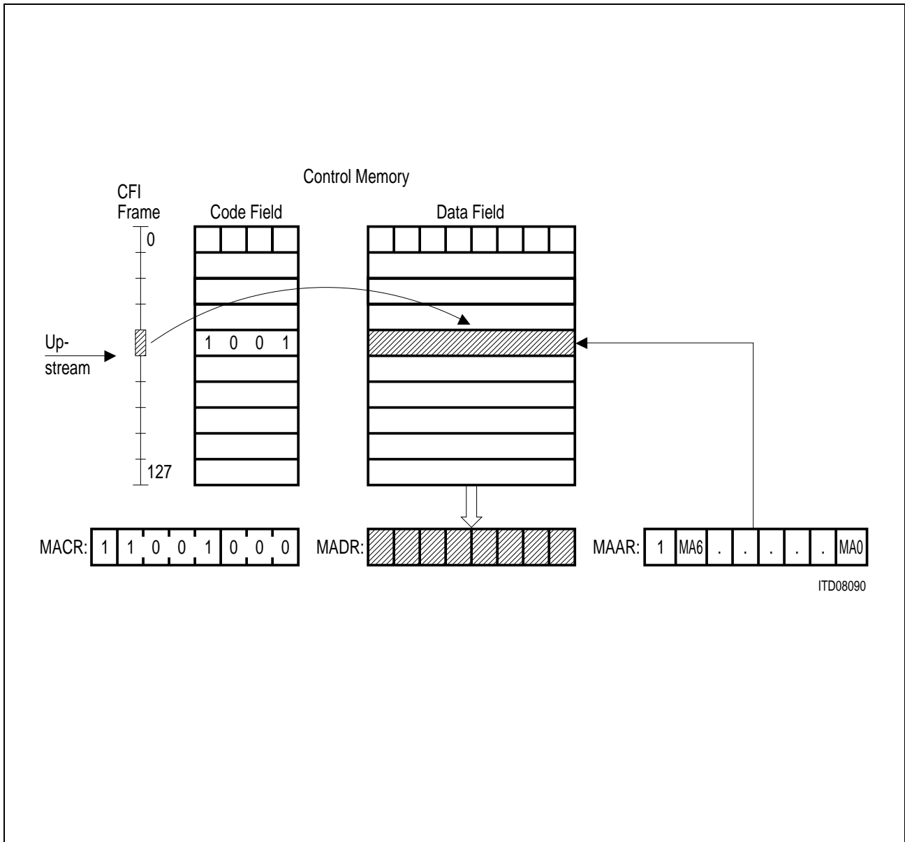
Figure 110 µP Access to the Upstream CFI Frame
