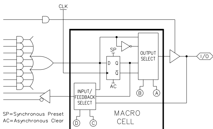
Figure 4 Block Diagram of the PEEL18CV8 I/O Macrocell
