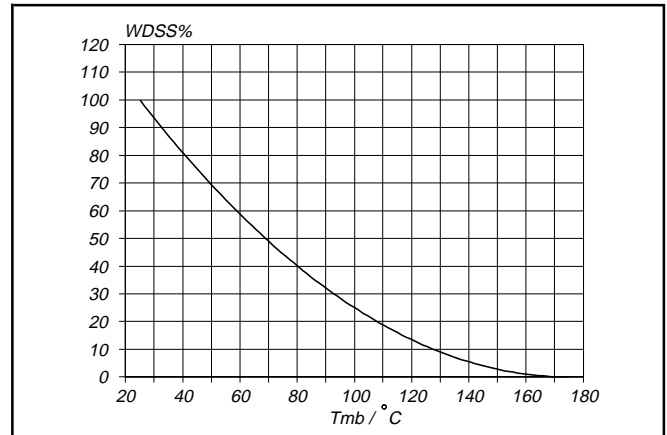
Fig. 15. Normalised avalanche energy rating. W_{DSS}\% = f(T_{mb}) ; conditions: I_D = 15 A
