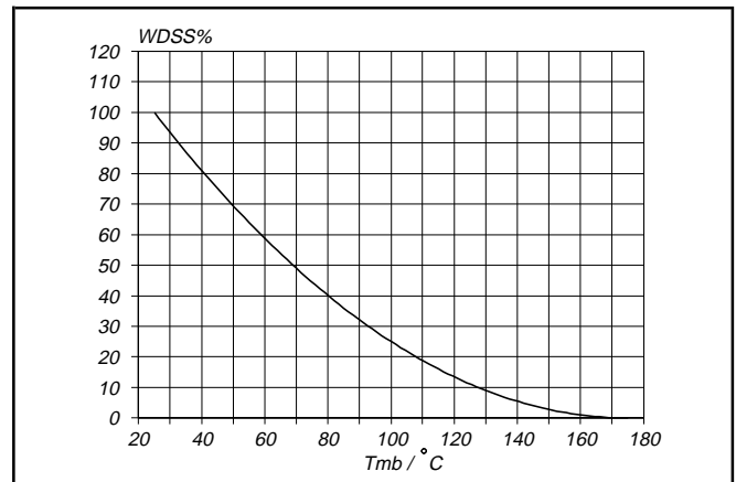
Fig. 15. Normalised avalanche energy rating. W_{DSS} \% = f(T_{mb}) ; conditions: I_D = 22 A
