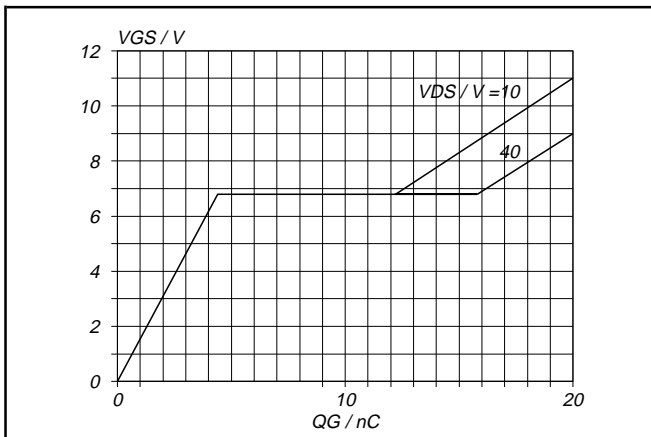
Fig. 13. Typical turn-on gate-charge characteristics. V_{GS} = f(Q_G) ; conditions: I_D = 22 A ; parameter V_{DS}
