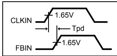
Figure 6. Propagation Delay
