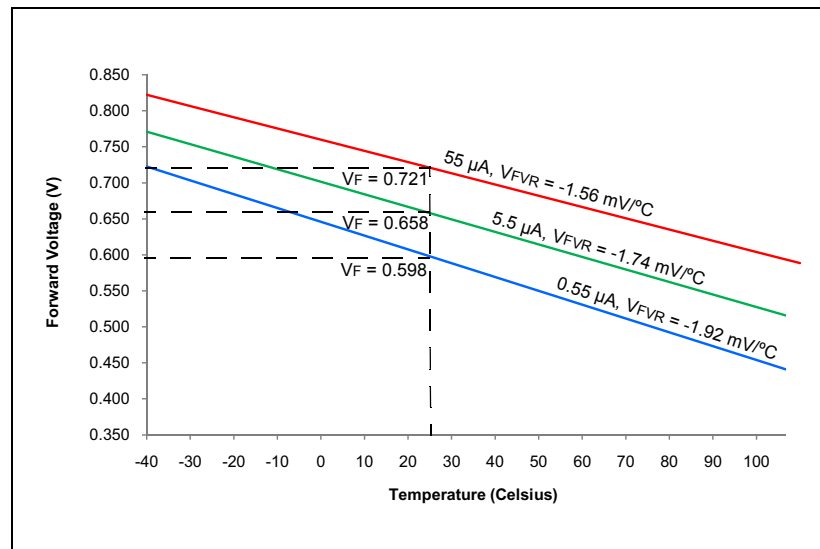
FIGURE 31-8: TYPICAL CTMU TEMPERATURE DIODE FORWARD VOLTAGE
