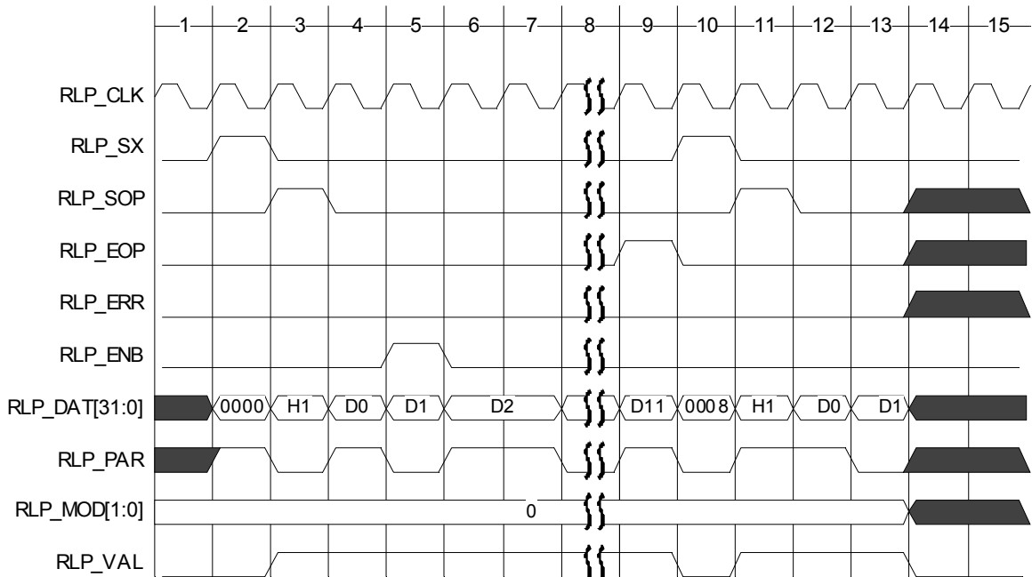
Figure 30 RxLink POS-PHY ATM Cell Transfer
