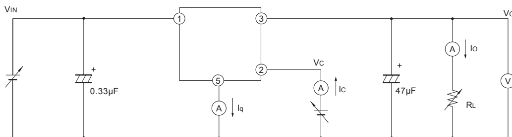
Fig.1 Test Circuit
