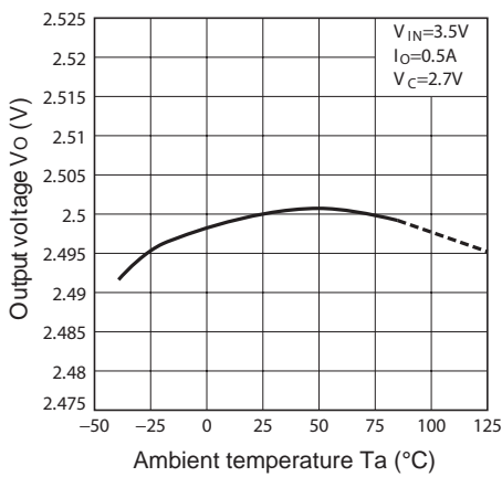
Fig.9 Output Voltage vs. Ambient Temperature (PQ025EH01ZxH)
