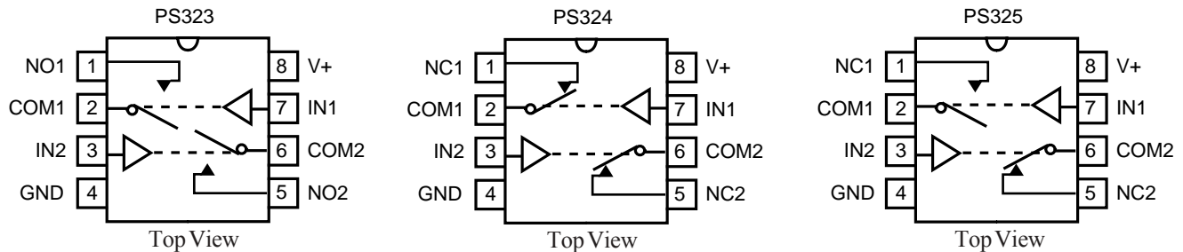
Switches shown for logic “0” input
