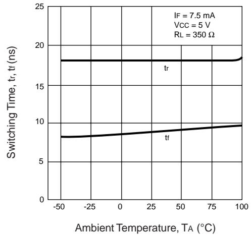
SWITCHING TIME vs. AMBIENT TEMPERATURE
