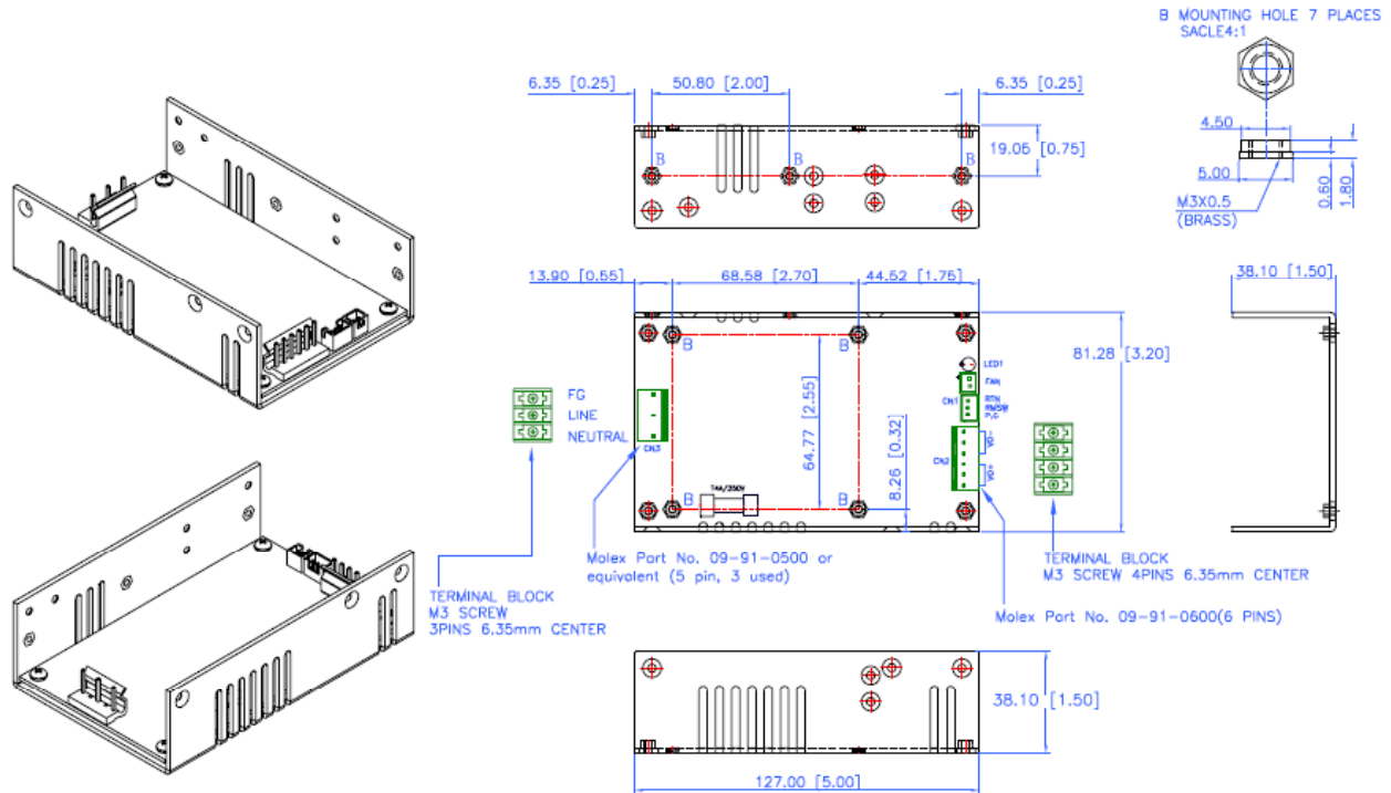
PSRL9827S Series (U-Chassis Type): 5(L) x 3.2(W) x 1.5(H) inches; Weight: 400g
