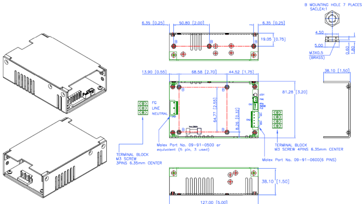
PSRL9827S Series (U-Chassis with Type A Cover): 5(L) x 3.2(W) x 1.56(H) inches; Weight: 420g
