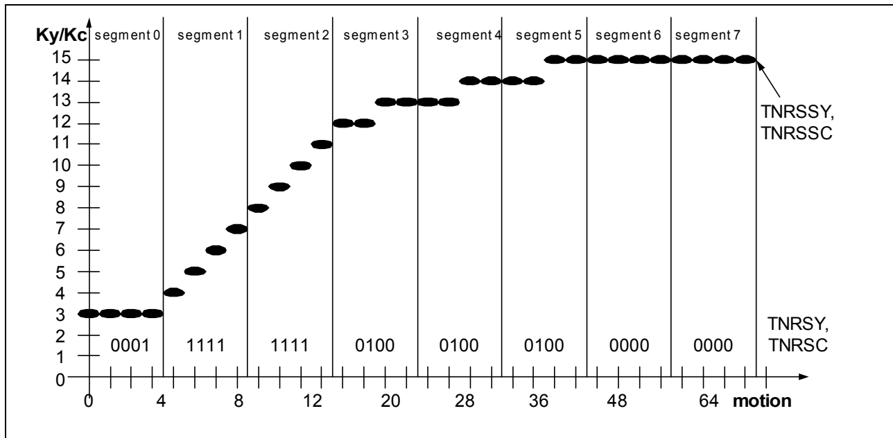
Figure 5-26 Predefined curve characteristics for LUT
