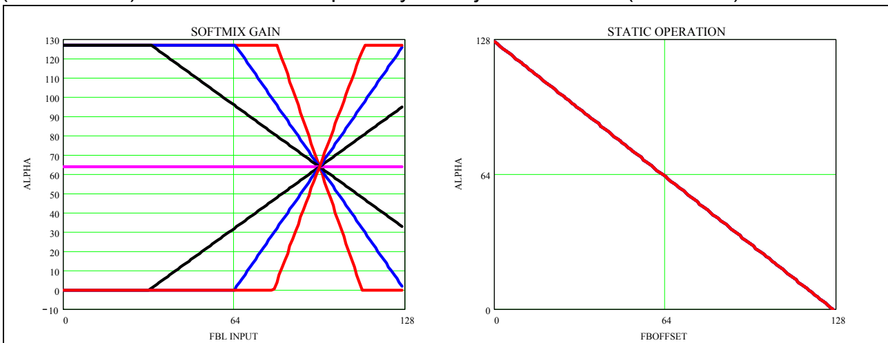
Figure 5-21 Varied FBOFFST output and static operation mode
