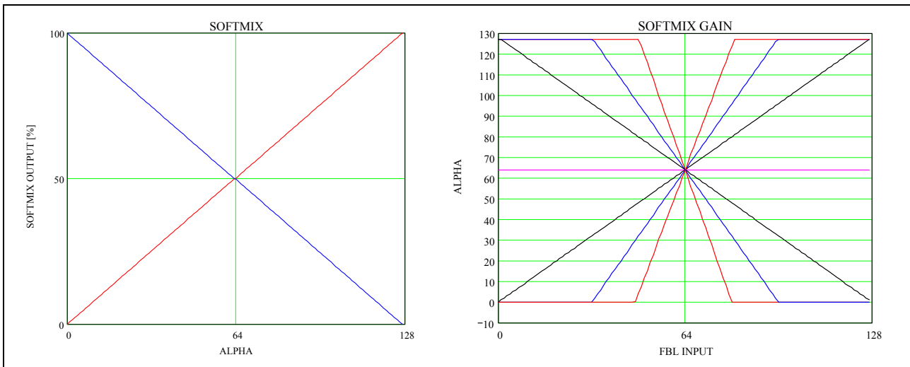
Figure 5-20 Softmix: Visualization of formulas
