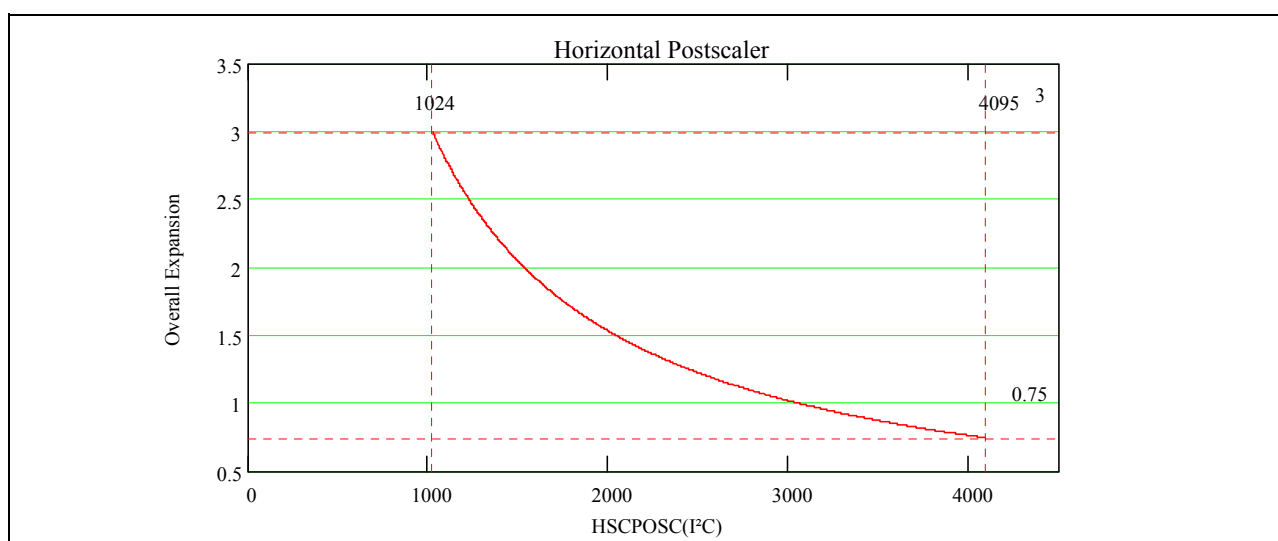
Figure 5-27 Expansion factor of horizontal postscaler dependent on HSCPOSC
