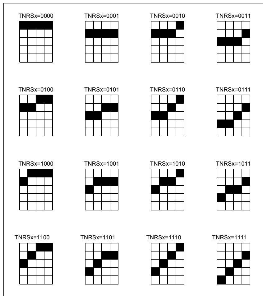
Figure 5-25 Segments of LUT
