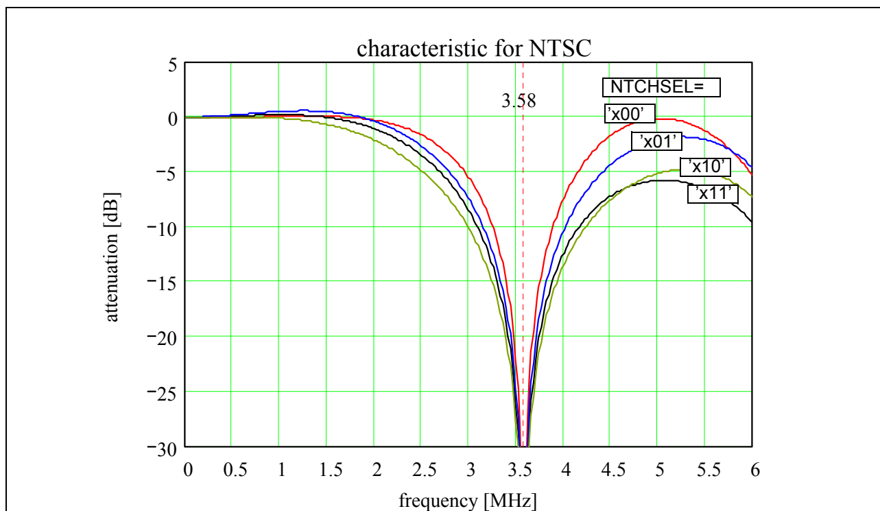
Figure 5-11 Filter characteristics for NTSC, PAL M and PAL N
