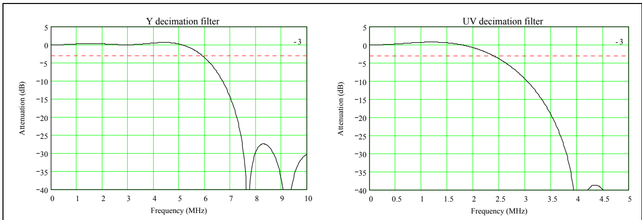
Figure 5-23 Y and C decimation filter characteristic for standard operation (1.5)
