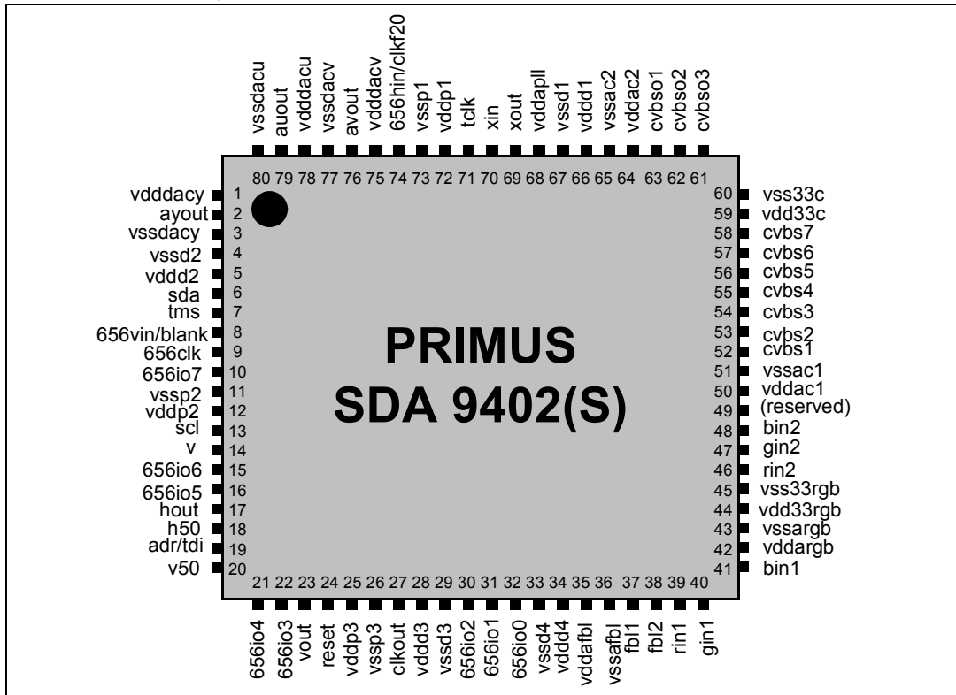
Figure 4-1 P-MQFP-80
