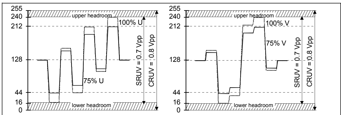
Figure 5-18 UV amplitude characteristics
