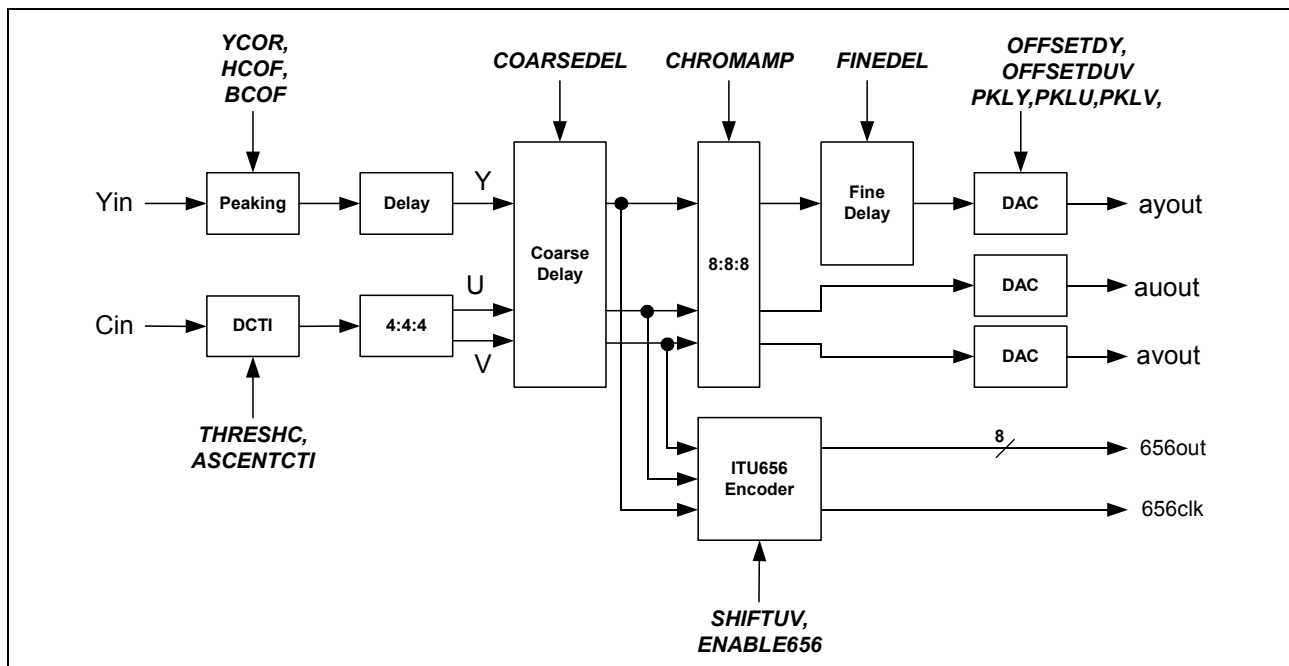
Figure 5-32 Block diagram of Display processing
