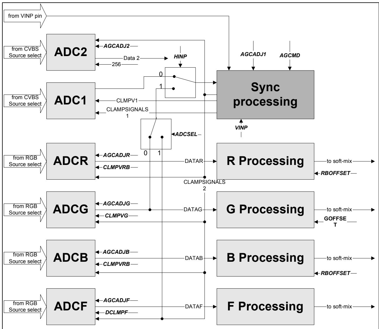
Figure 5-16 Signal and Clamping organization
