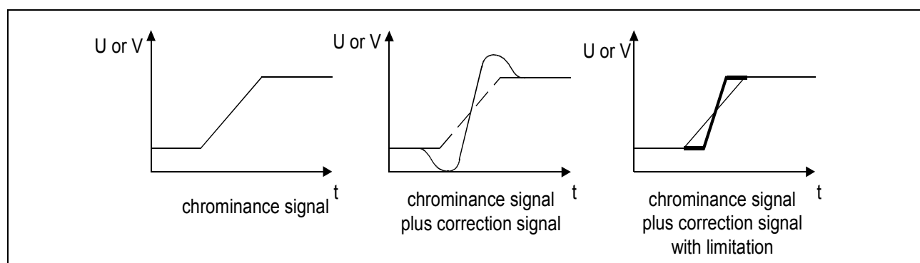
Figure 5-35 Principles of DCTI
