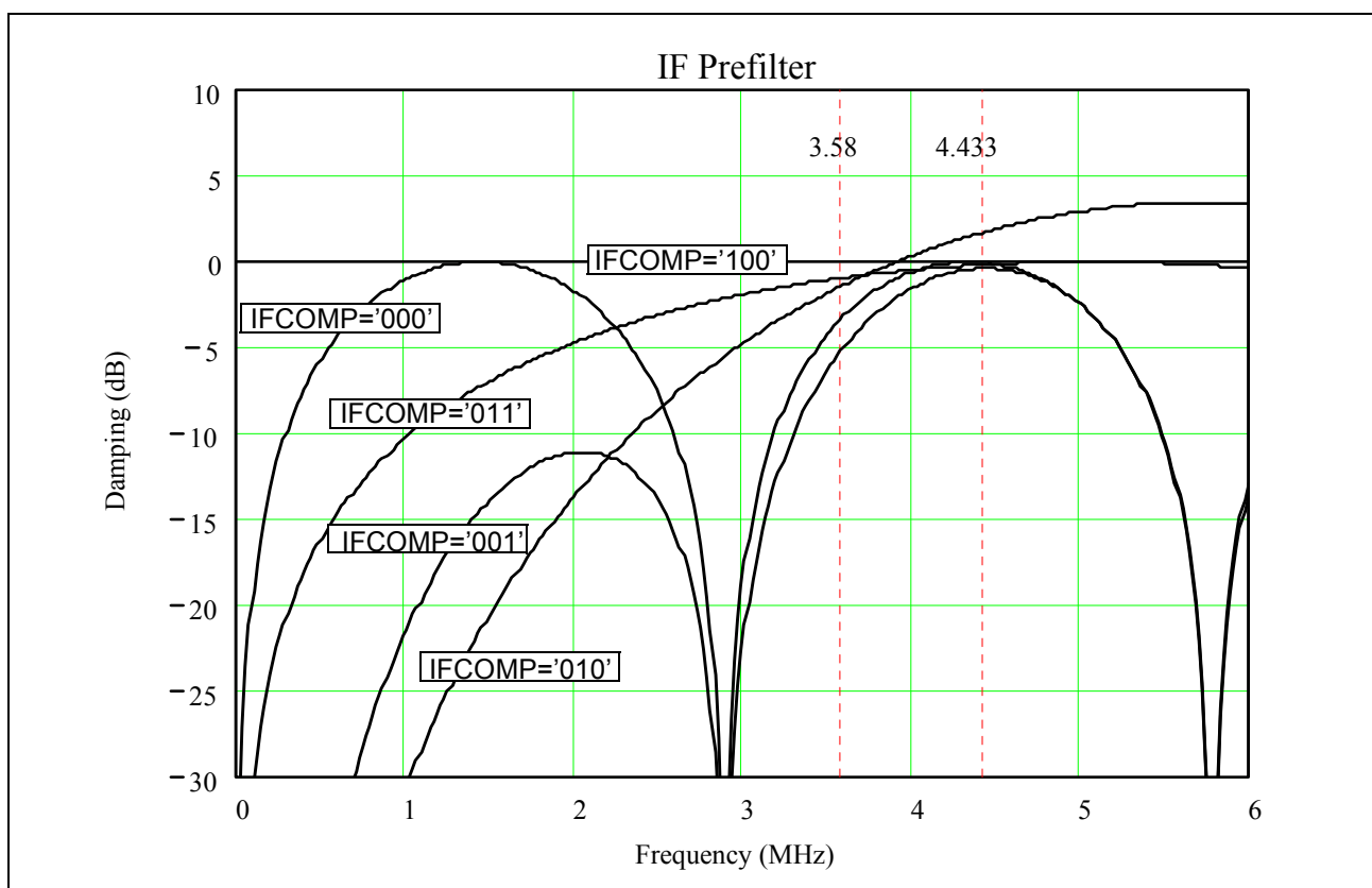
Figure 5-8 IF prefilter
