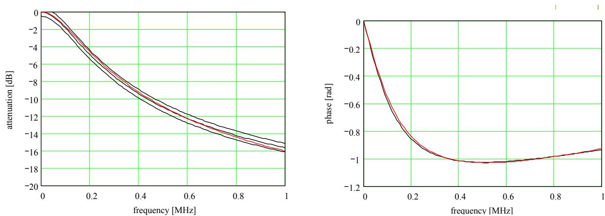
Figure 5-10 Bell filter (baseband): standard (black) and implementation (red)
