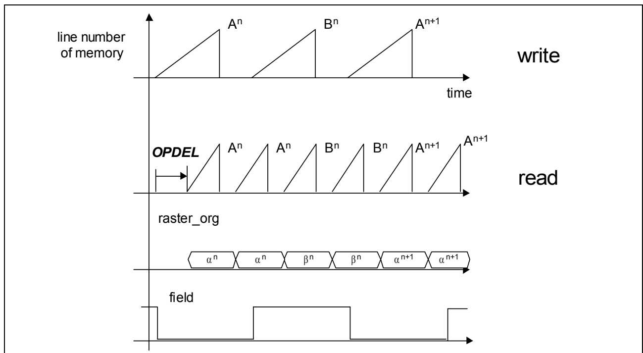
Figure 5-31 50/60 Hz interlaced to 100/120 Hz interlaced conversion (AABB)
