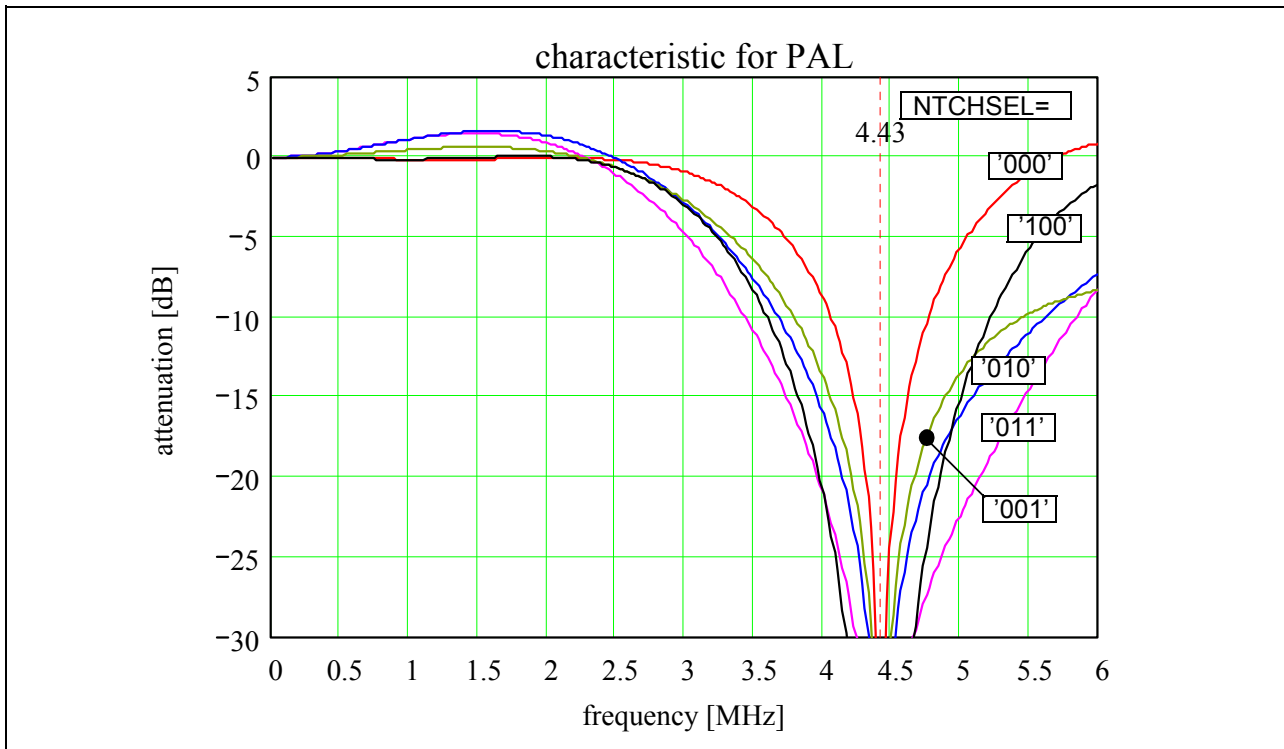
Figure 5-12 Filter characteristics for PAL B/G, NTSC44, PAL60
