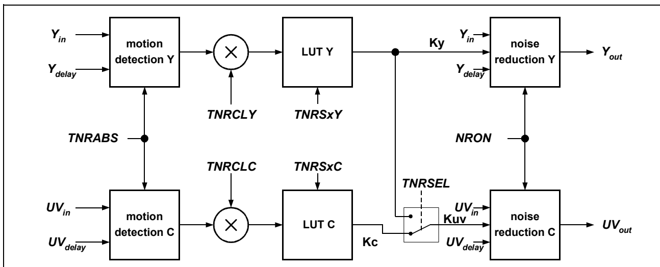
Figure 5-24 Temporal noise reduction
