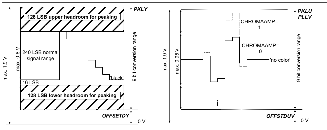
Figure 5-36 DAC output signals
