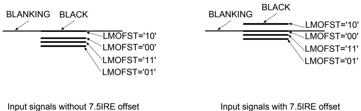
Figure 5-15 Adjustment of 'Black-' to 'Blankingvalue' at analog output
