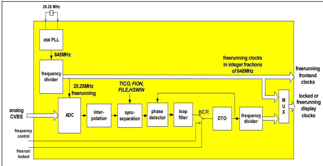
Figure 5-41 Linelocked clock generation
