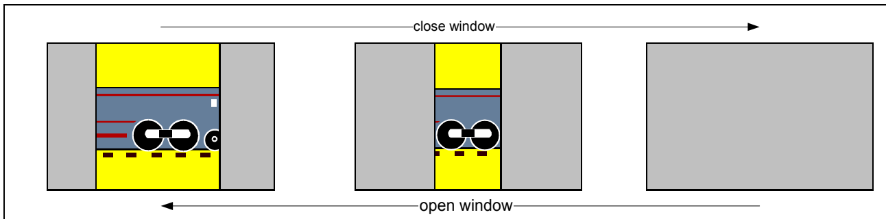
Figure 5-38 Horizontal windowing
