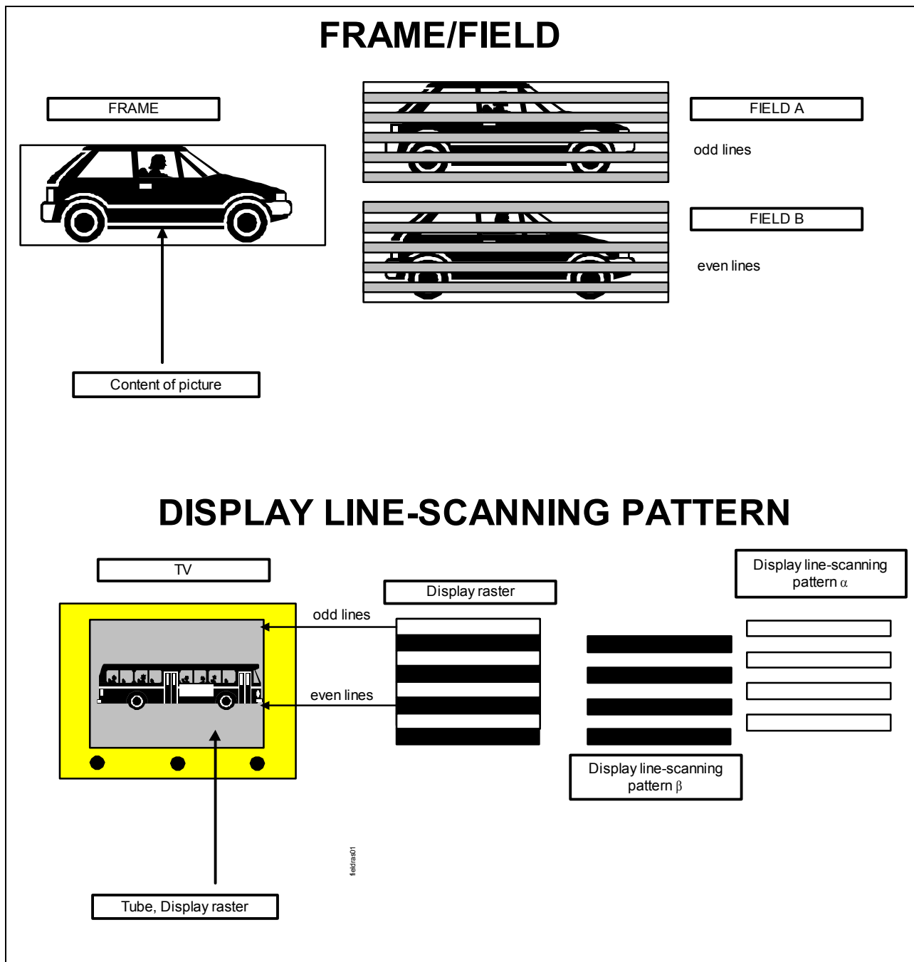
Figure 5-30 Explanation of field and display line-scanning pattern
