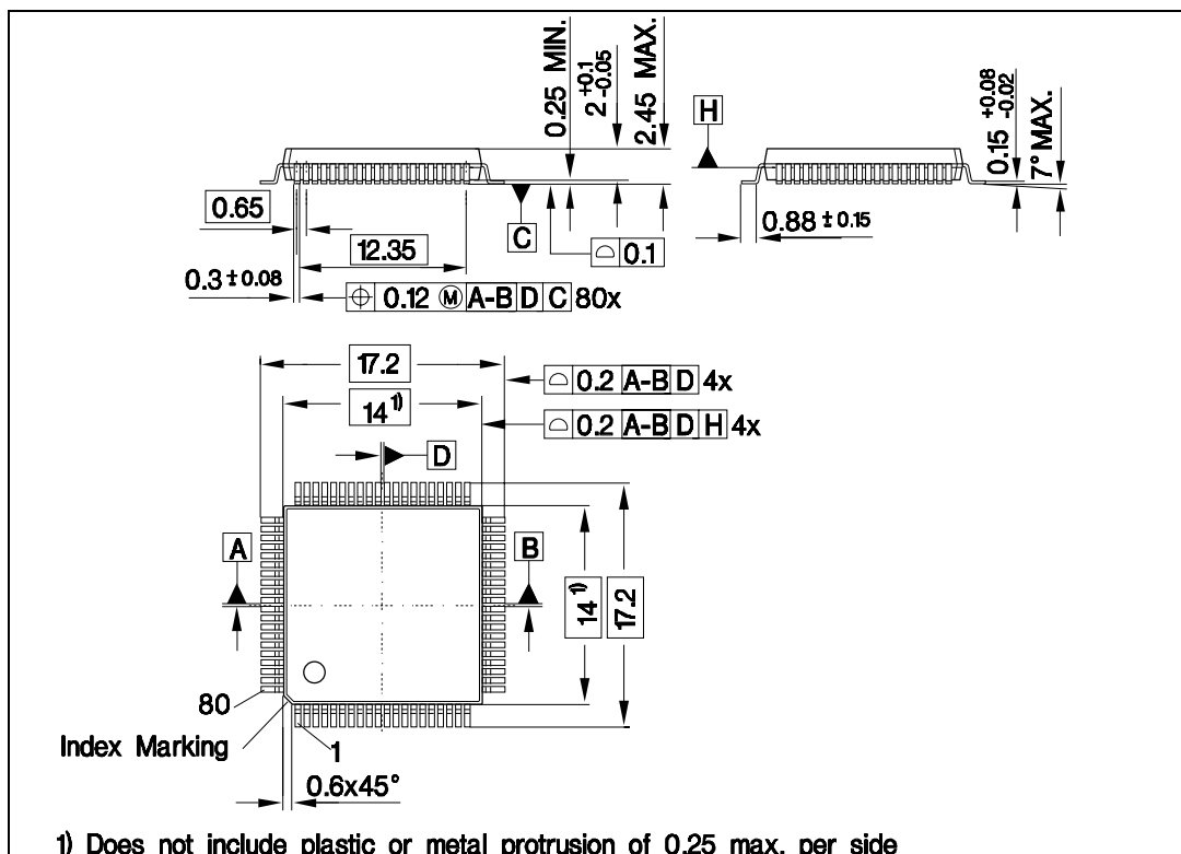
Figure 4-2 Package outlines P-MQFP-80
