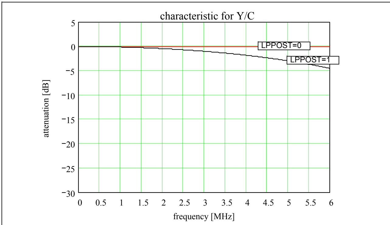
Figure 5-14 Filter characteristics for Y/C mode
