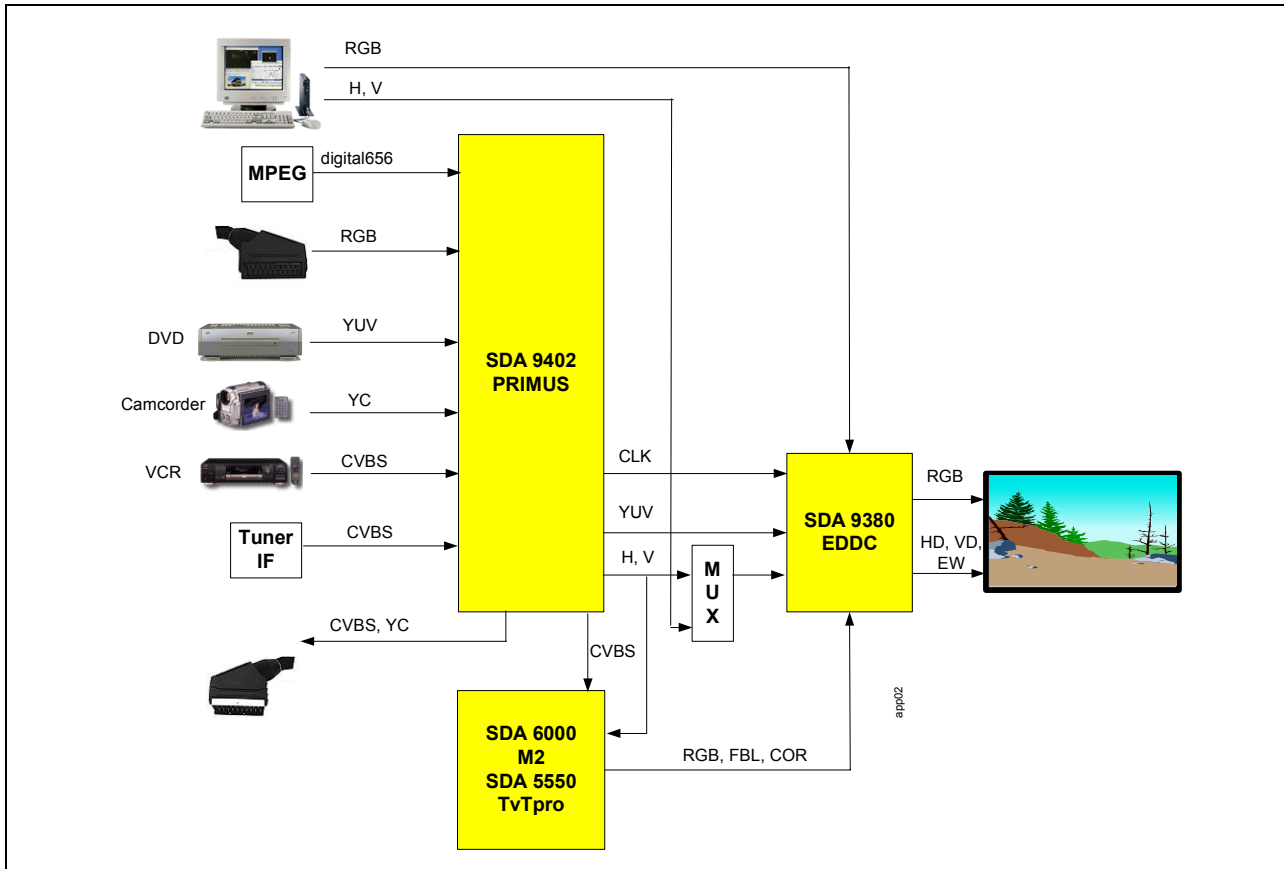
Figure 12-2 Application Overview
