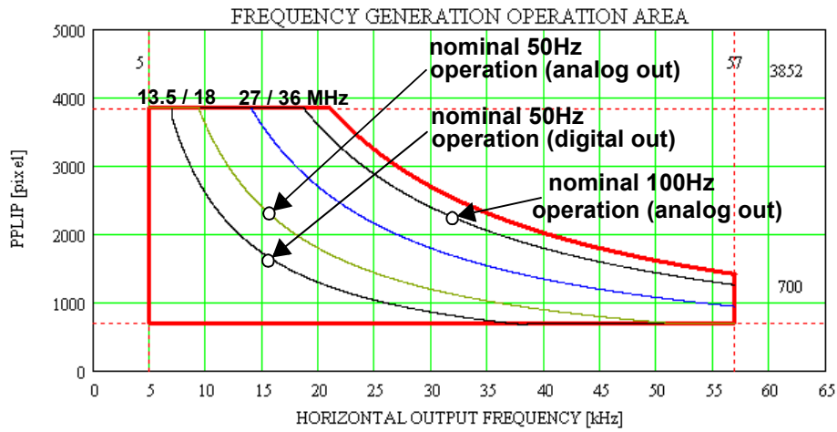
Figure 5-42 Allowed operation area for clock generation
