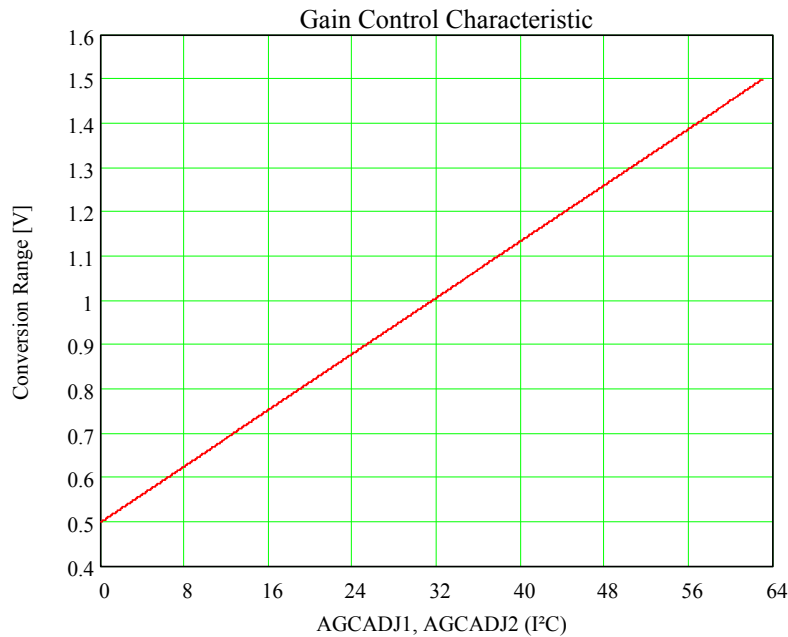
Figure 5-2 CVBS ADC characteristic
