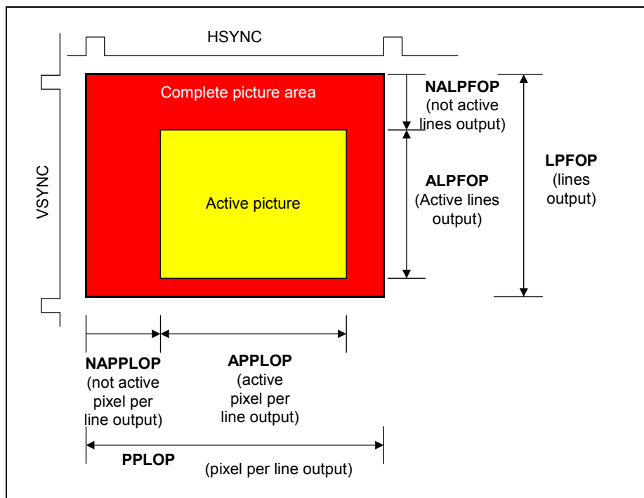
Figure 5-37 Image format behind memory
