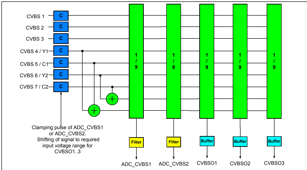
Figure 5-1 Input selection
