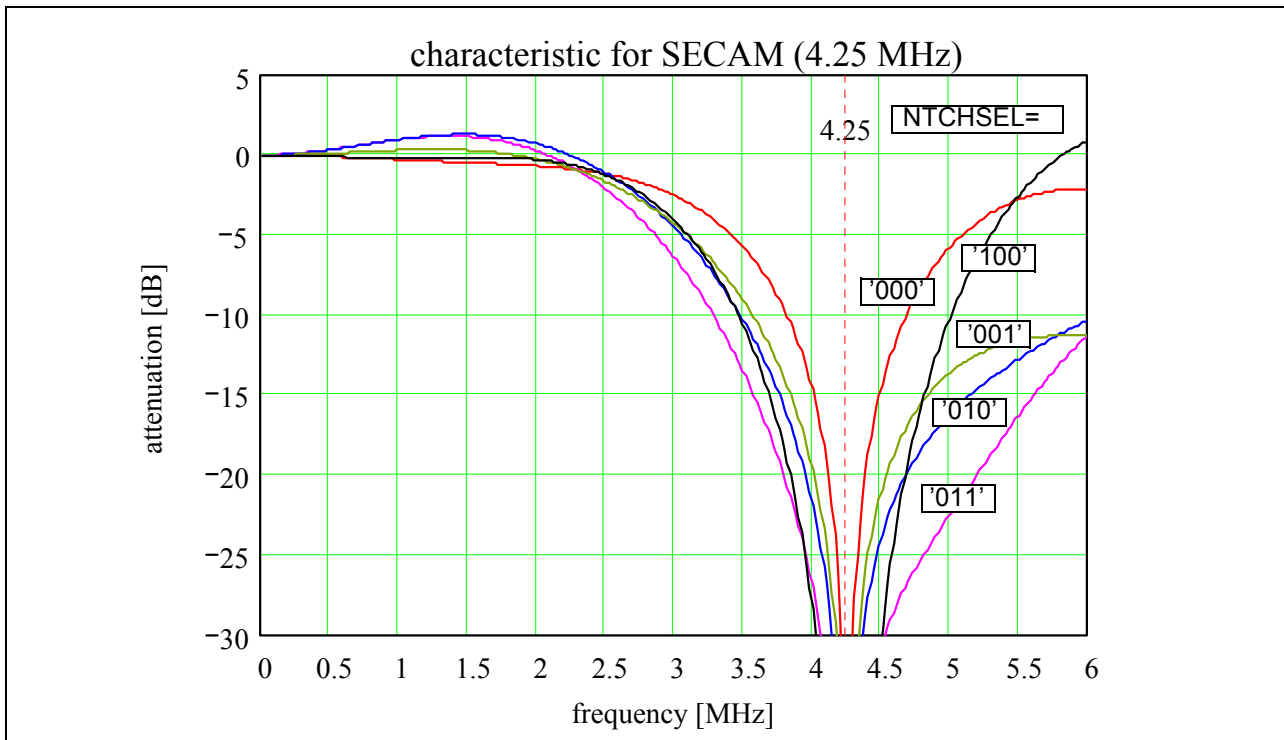
Figure 5-13 Filter characteristics for SECAM (SECNTCH='01', 4.25 MHz)
