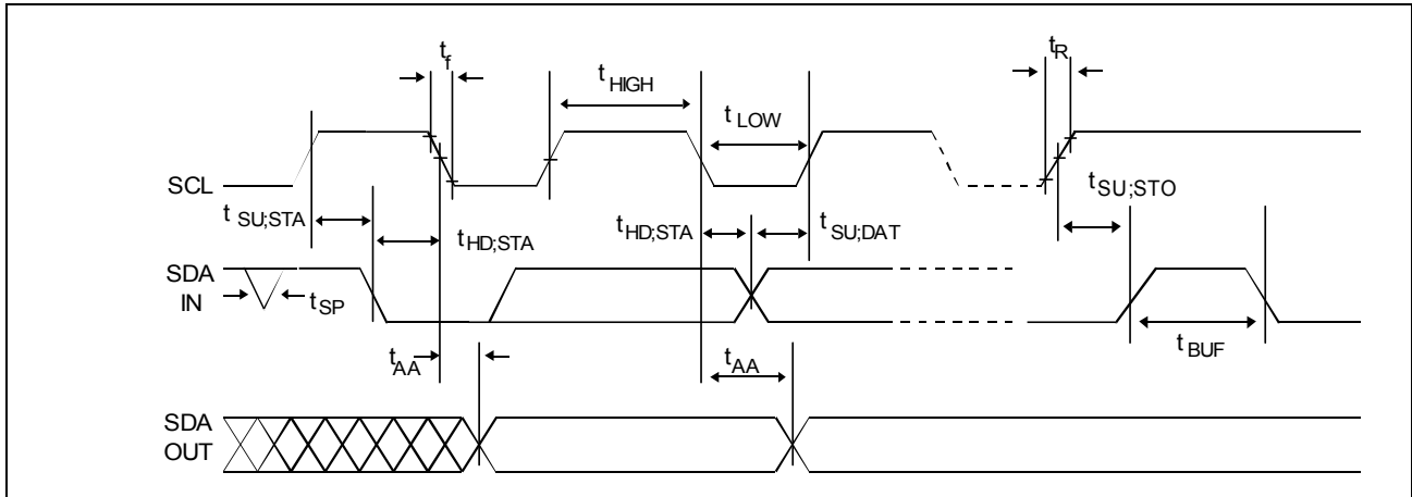
Figure 11-1 I 2 C bus timing data
