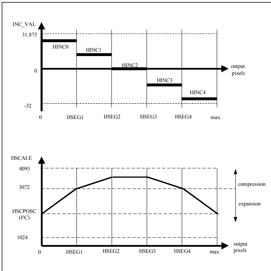
Figure 5-28 Visualization of panorama segments
