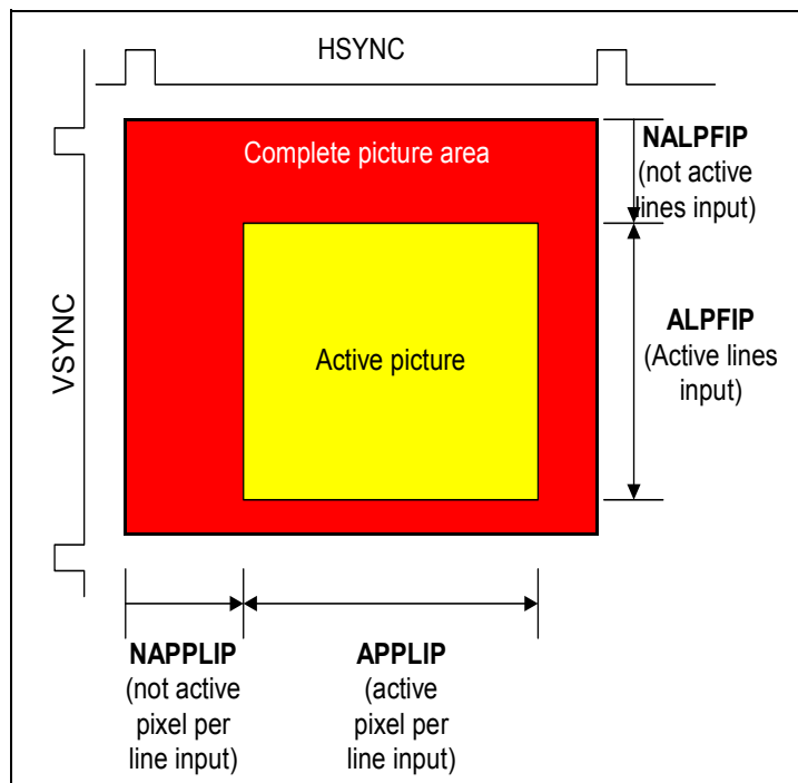
Figure 5-22 Image format before memory
