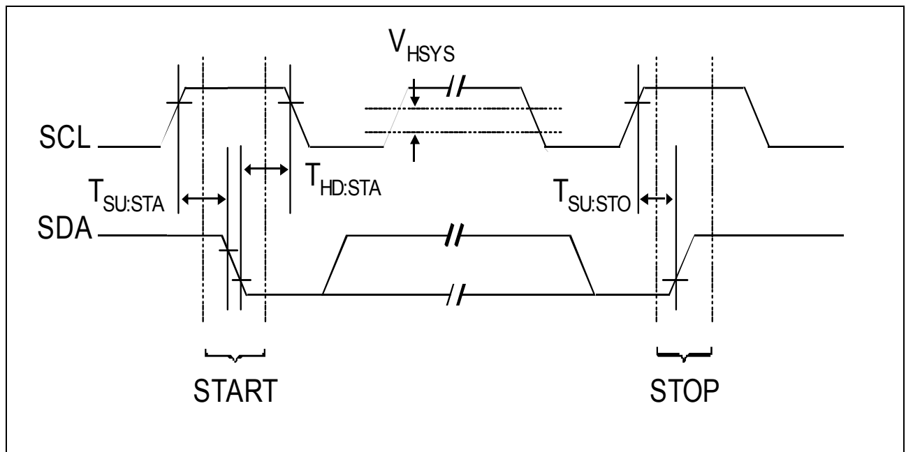
Figure 11-2 I 2 C Bus timing start/stop
