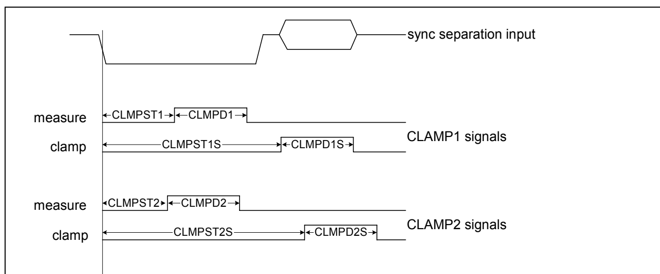
Figure 5-4 Clamping signals
