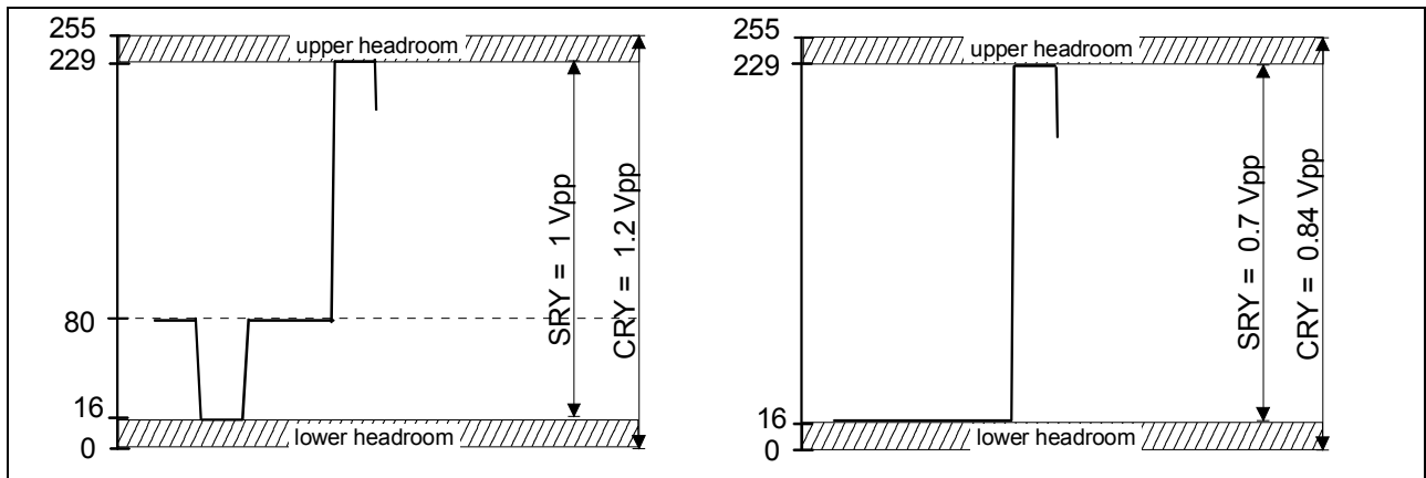
Figure 5-17 Y/RGBF amplitude characteristics (with or without sync)
