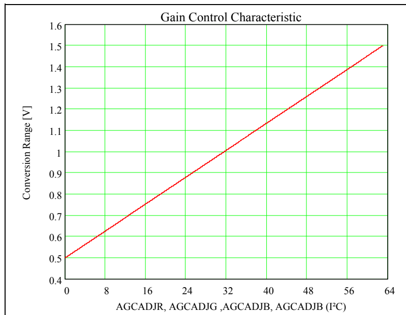
Figure 5-19 RGBF ADC characteristic
