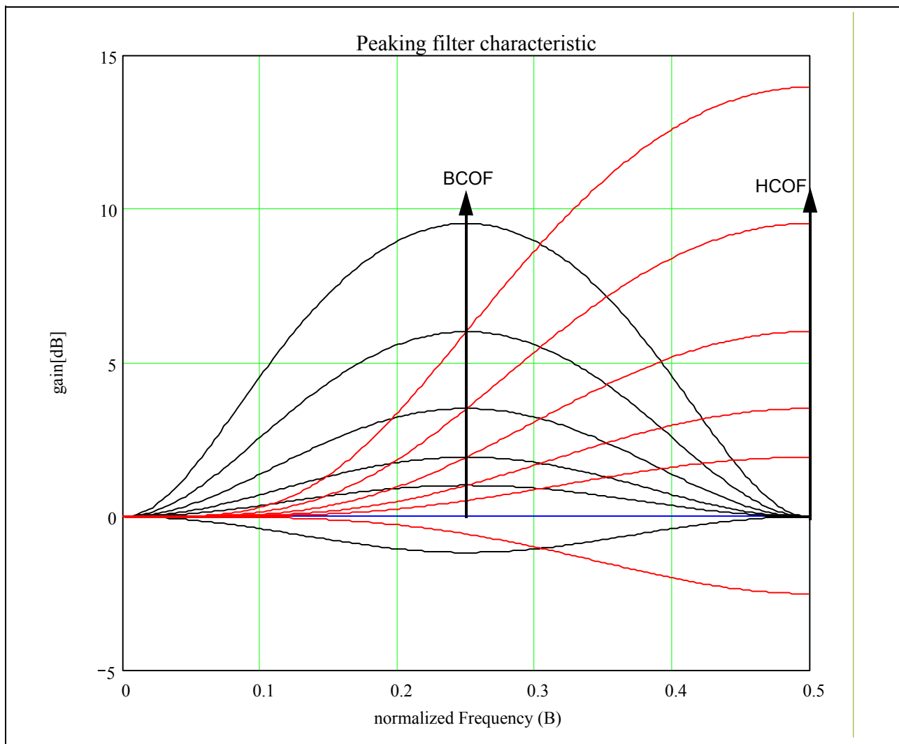
Figure 5-34 Peaking filter: Bandpass and Highpass filter
