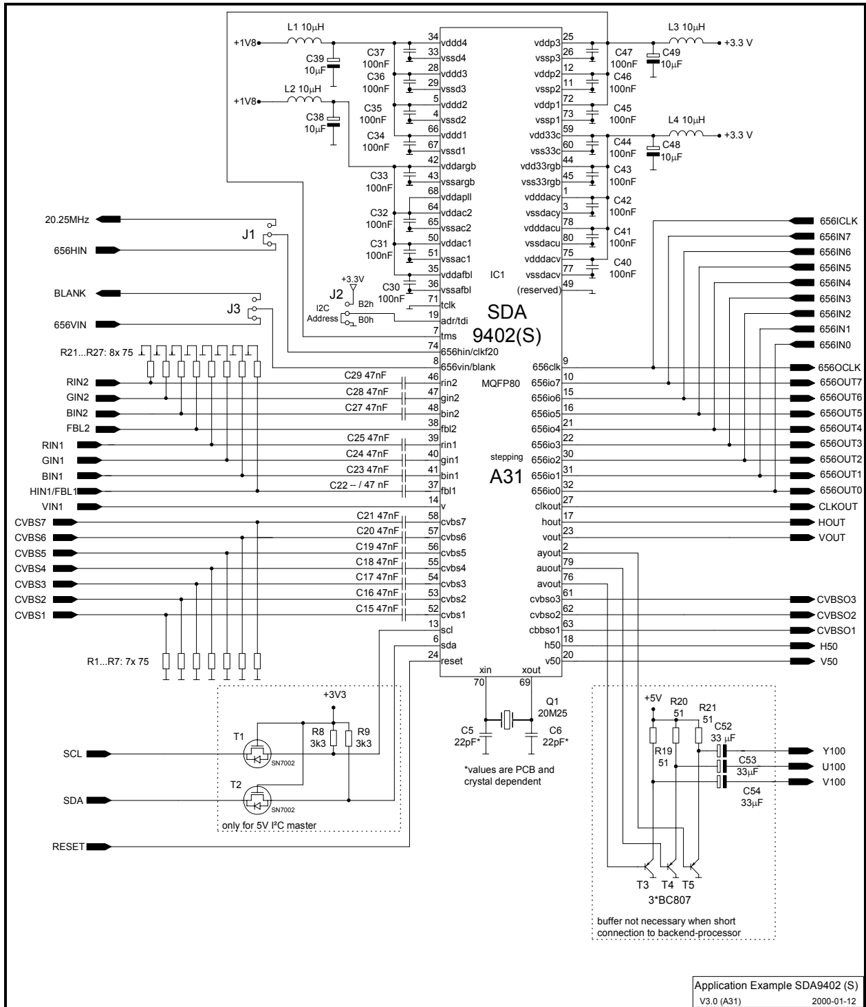
Figure 12-1 Application Example SDA9402(S)
