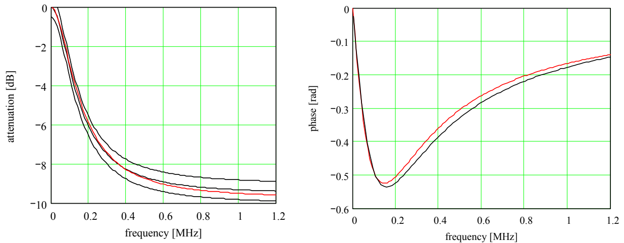
Figure 5-9 Deemphase filter: standard (black) and implementation (red)
