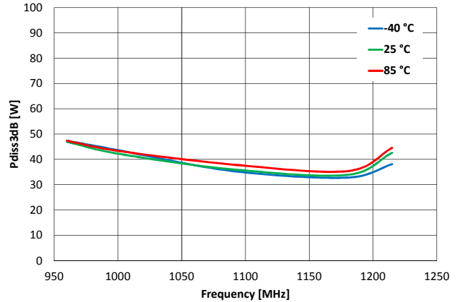
Pdiss3dB Over Temperatures
