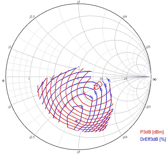
Load Pull at 2.17 GHz
