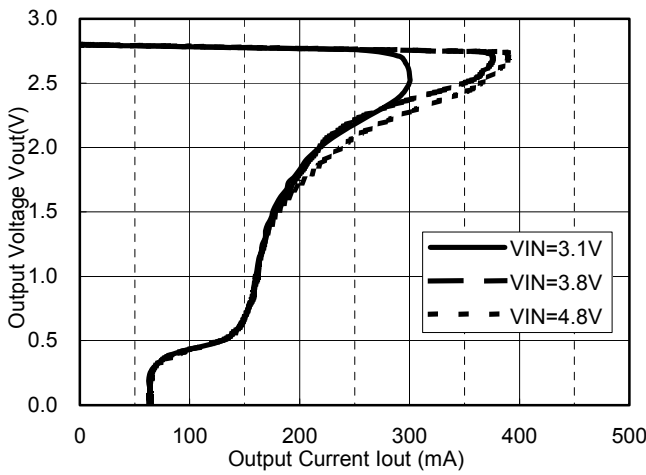
V_{OUT}=2.8V
