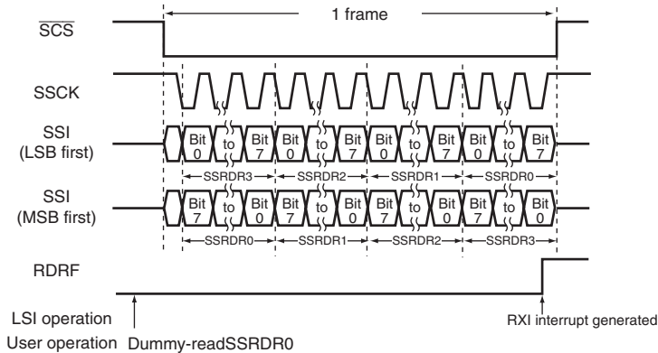
Figure 18.7 Example of Reception Operation (SSU Mode)
