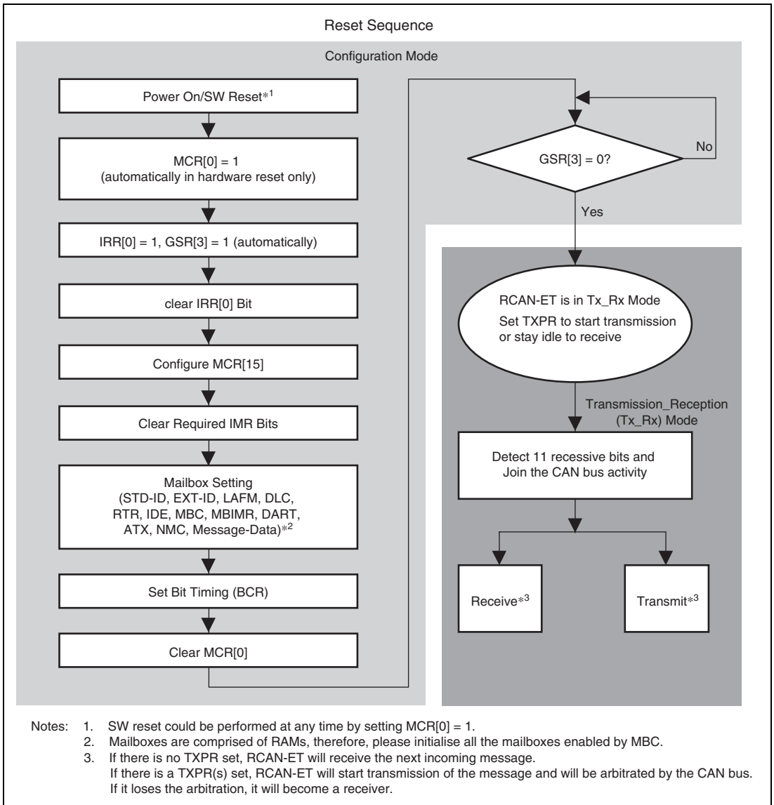
Figure 22.8 Reset Sequence
