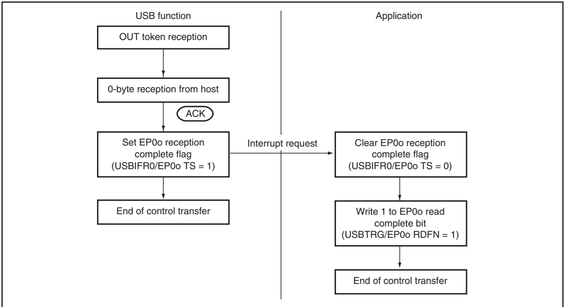
Figure 25.8 Status Stage (Control-IN) Operation
