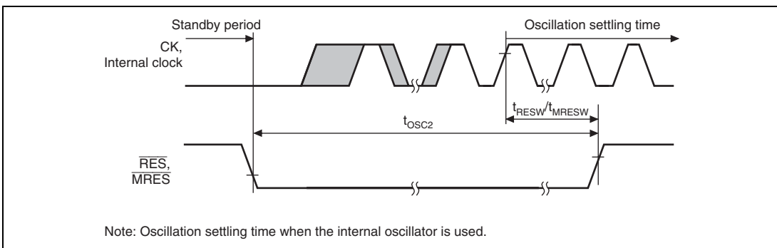
Figure 31.5 Oscillation Settling Time on Return from Standby (Return by Reset)
