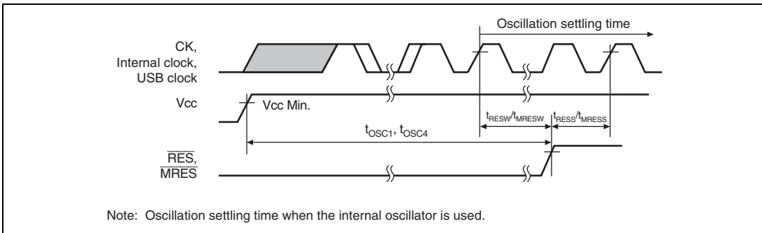
Figure 31.4 Power-On Oscillation Settling Time
