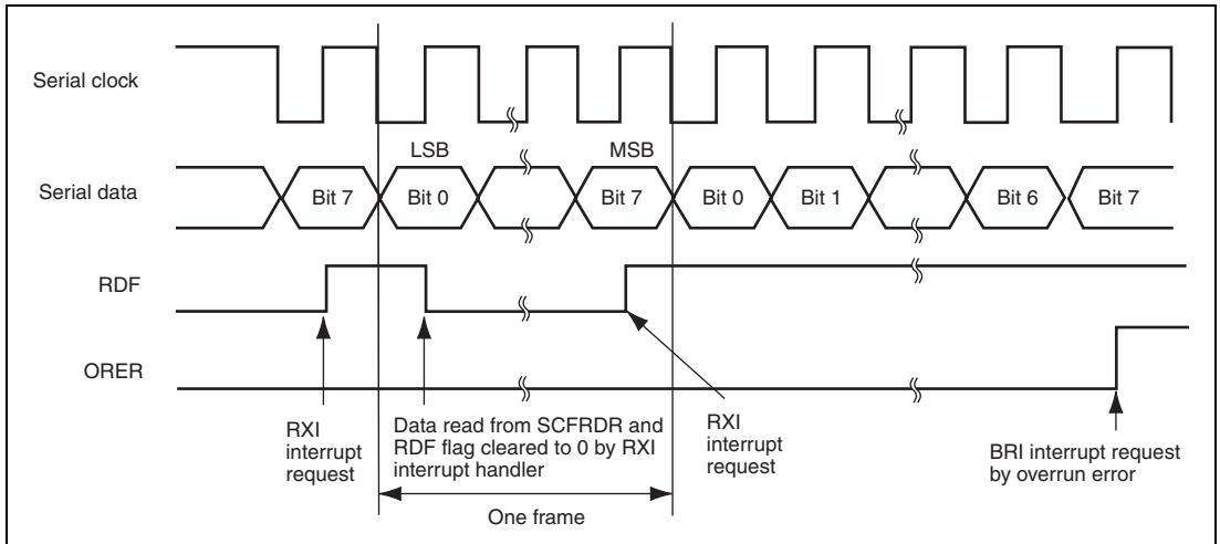
Figure 17.15 Example of SCIF Receive Operation
