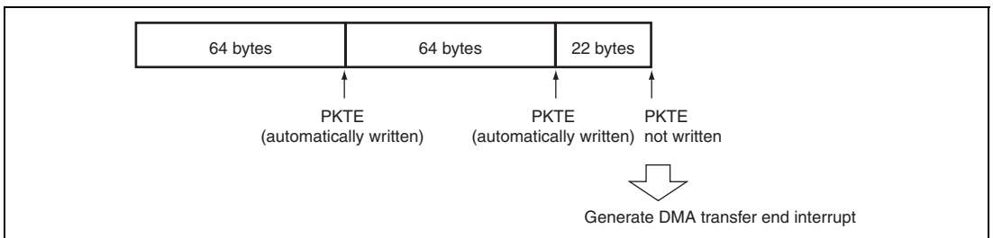
Figure 25.18 EP2 PKTE Operation
