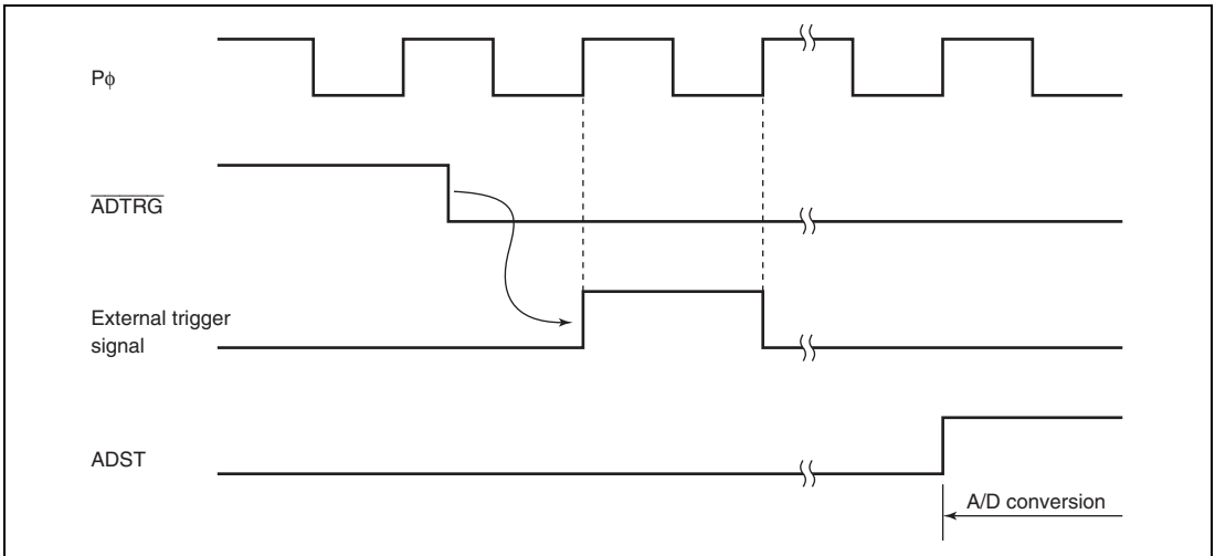
Figure 20.11 External Trigger Input Timing
