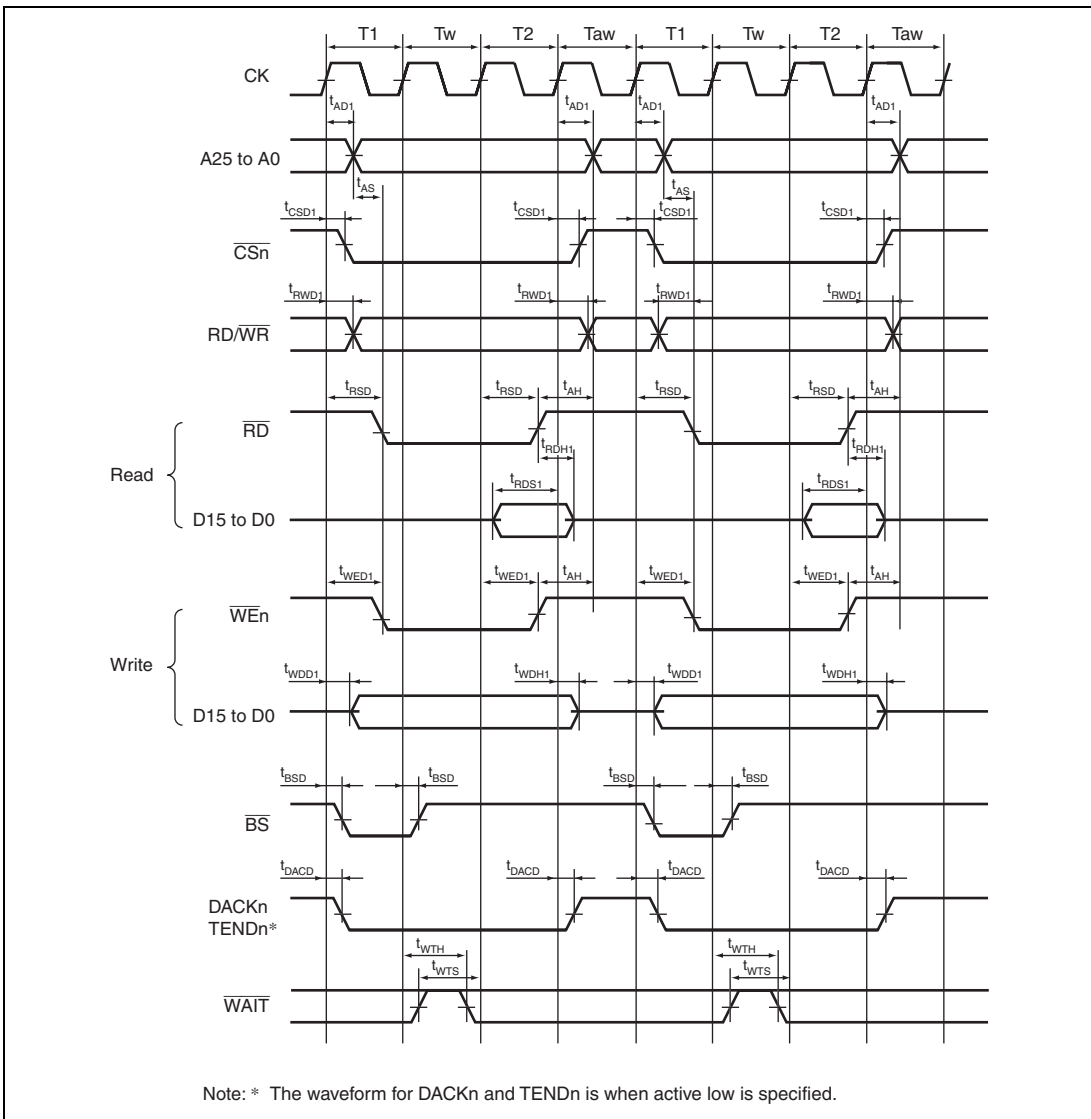
Figure 31.14 Basic Bus Timing for Normal Space (One Software Wait Cycle, External Wait Cycle Valid (WM Bit = 0), No Idle Cycle)
