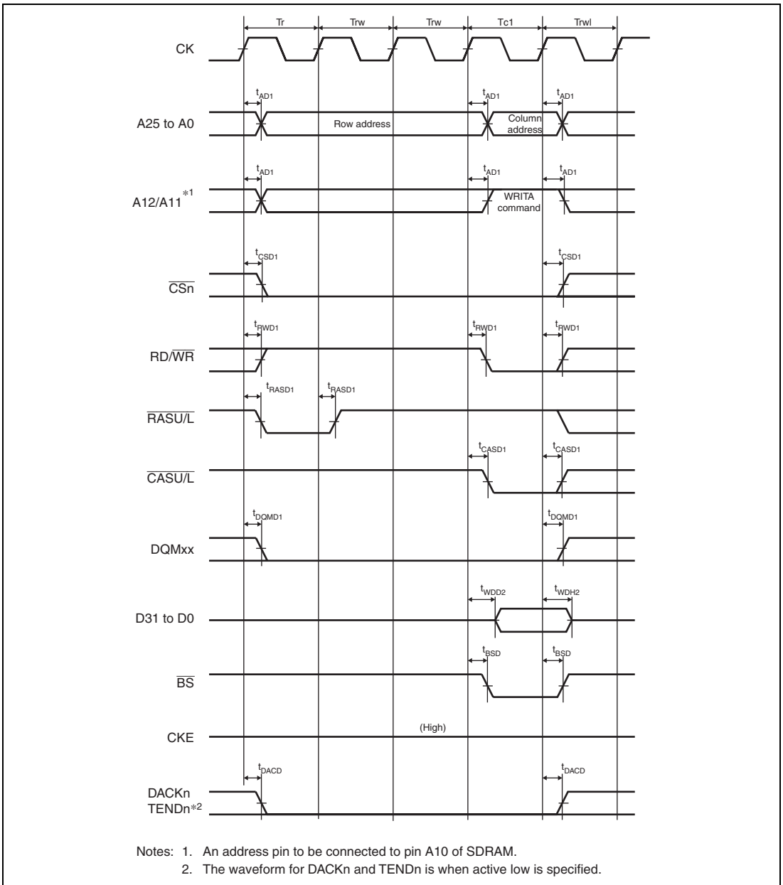
Figure 31.24 Synchronous DRAM Single Write Bus Cycle (Auto Precharge, WTRCD = 2 Cycles, TRWL = 1 Cycle)
