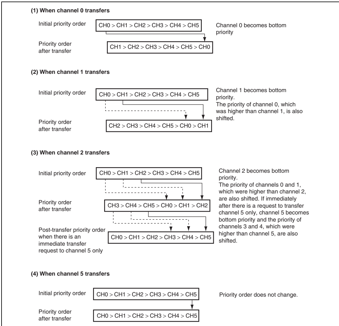
Figure 12.2 Round-Robin Mode
