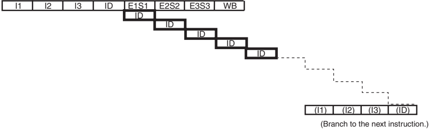
Figure 4.2 Instruction Execution Patterns (4)
