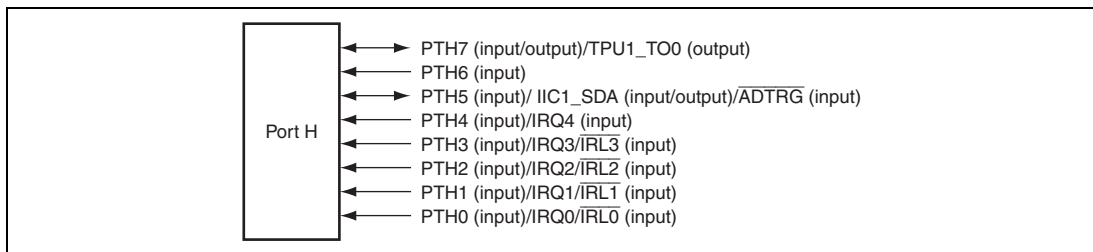
Figure 28.8 Port H
