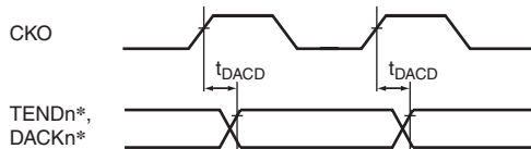
Figure 33.42 TEND, DACK Output Timing
