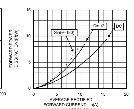
I_o - P_f CHARACTERISTICS
