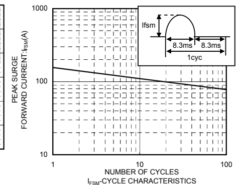
I_{FSM} CYCLE CHARACTERISTICS
