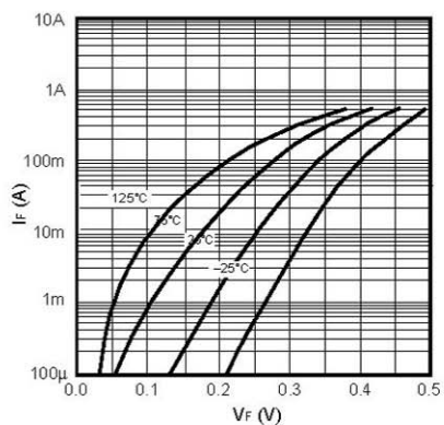
Fig.1 Forward characteristics
