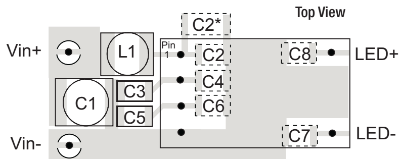
Recommended PCB Layout for Pinned / SMD Versions
