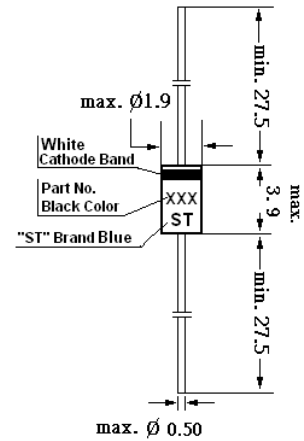
Glass case JEDEC DO-35 Dimensions in mm
