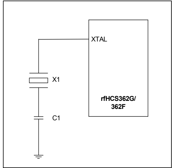
FIGURE 6-1: EXAMPLE ASK EXTERNAL CRYSTAL CIRCUIT
