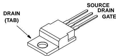
TO-220AB
